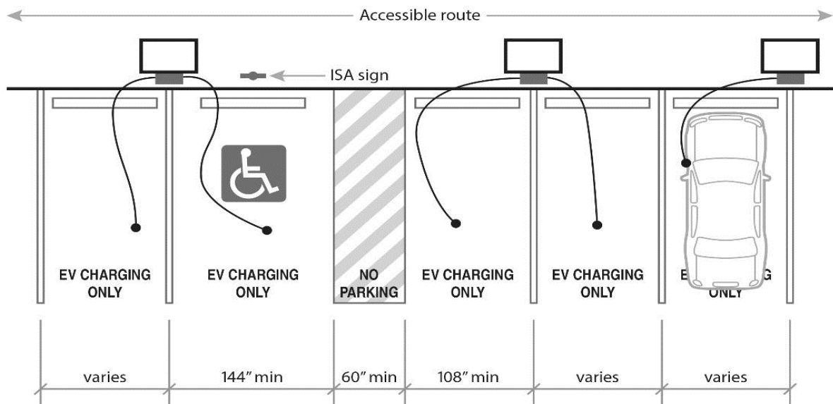
Example of Non-Residential EVSE Configuration
