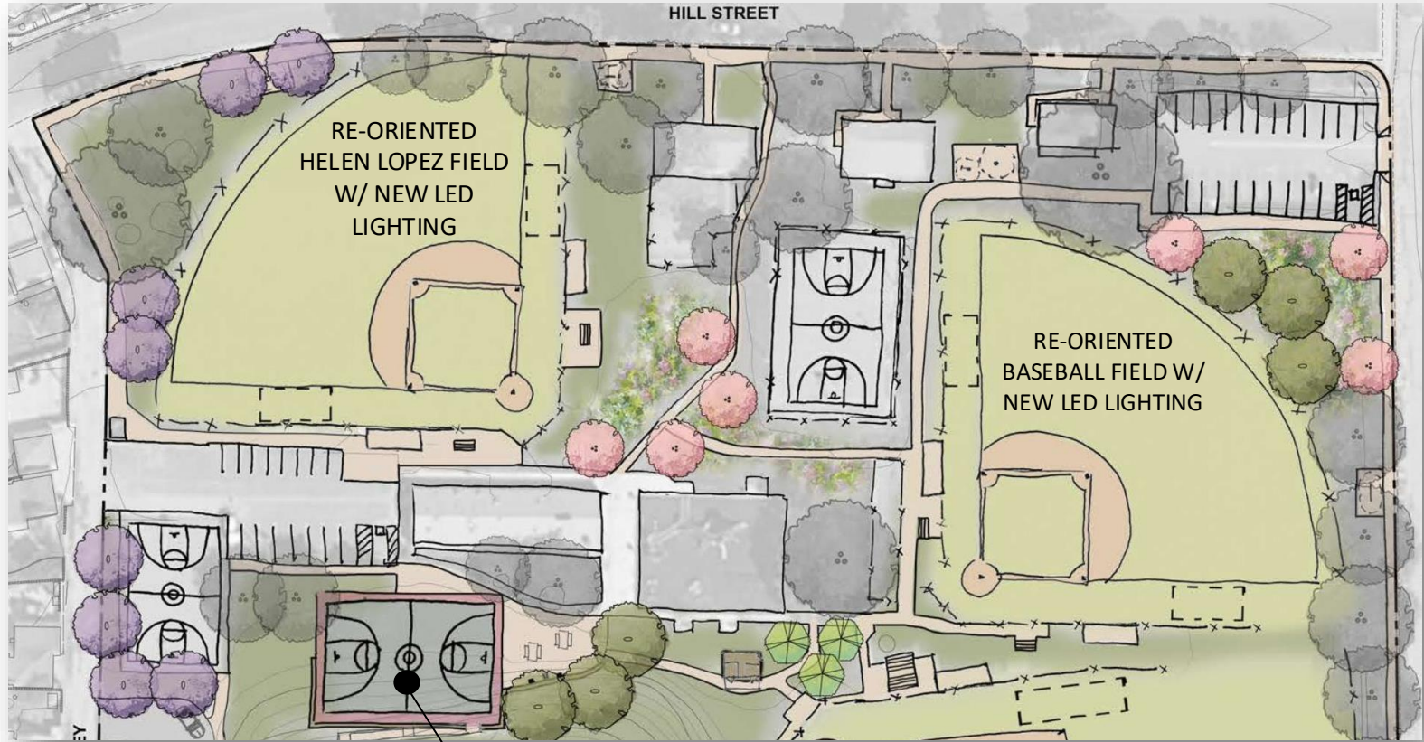
50'X94' NEW BASKETBALL COURT WITH NEW LED LIGHTING
