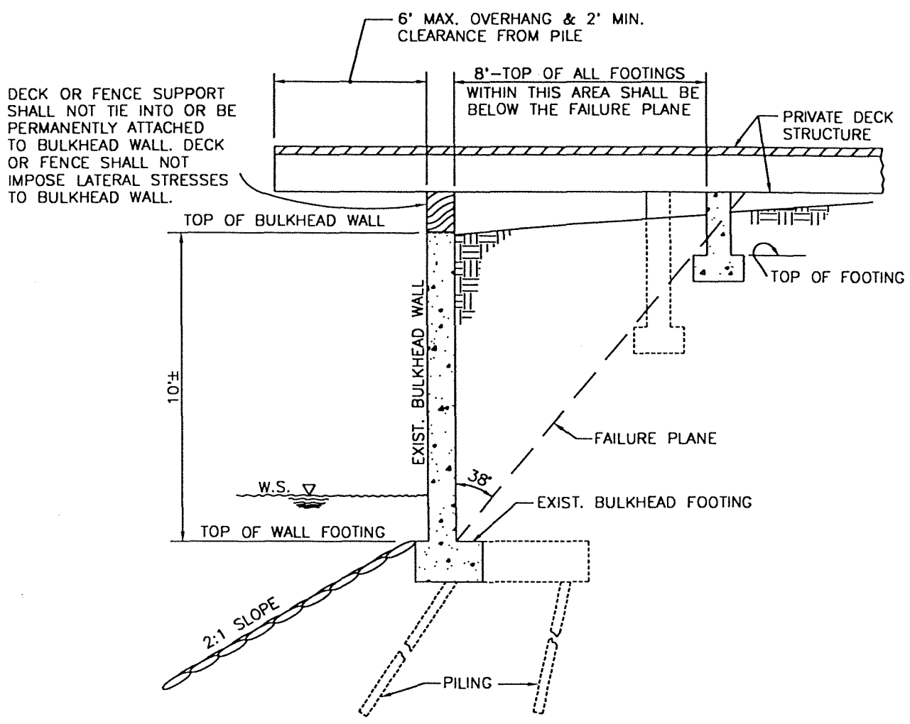
TYPICAL SECTION
