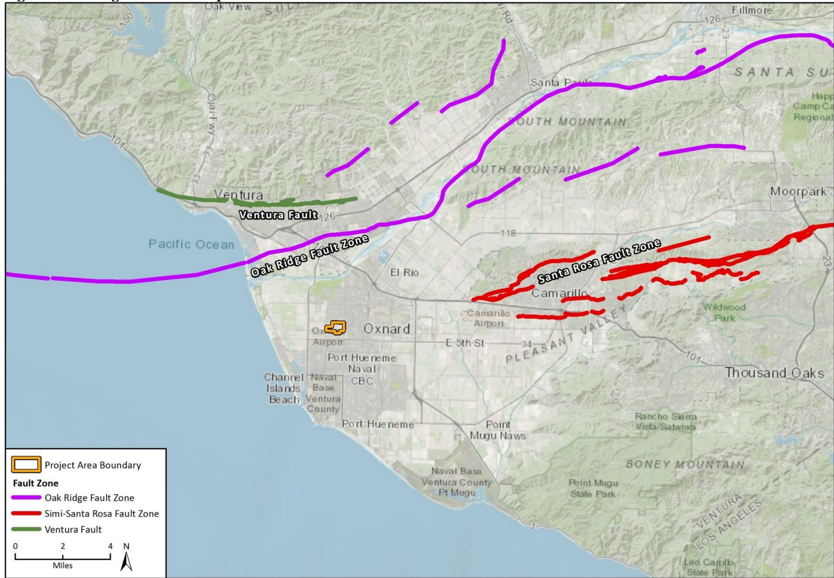
Figure 4.5-1 Regional Fault Map
